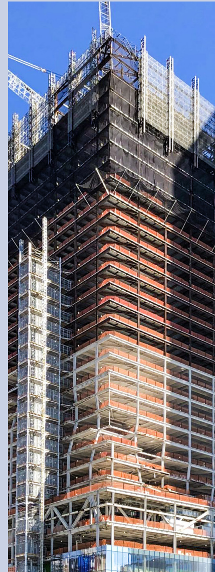
SPIRAL TOWER 66 Hudson Yards, New York City, U.S.A. Benson provided a 460-ton steel-mesh Cocoon. This technology hydraulically crawls up the sides of the building as they erect structural steel around the tower's core. Driven by its own power, the cocoon travel between floors without the aid of a crane making a protective shell for workers, equipment and parts that makes skyscraper construction safer and faster.
